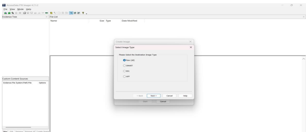
Figure 3: Configuring the destination image format to Raw (dd)
